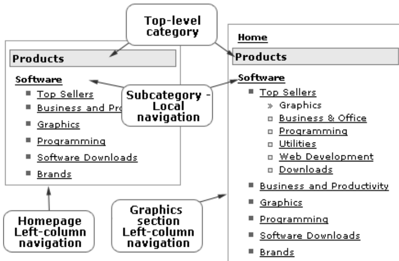
Figure 8.16. Complementary global and local navigation
